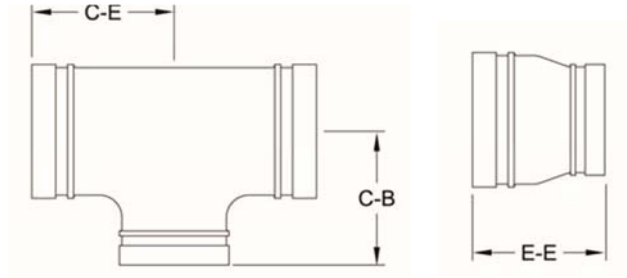
Model SS-21 Reducing Tee, SS-50 Concentric Reducer
