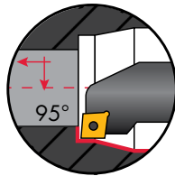
boring & facing
