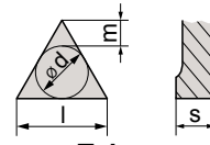
Tolerance d ± 0.003 m ± 0.005 s ± 0.005
