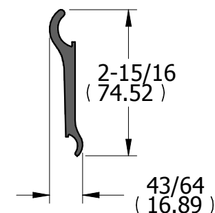
WRENCH
