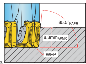
WEP - See insert drawing for wiper options.
